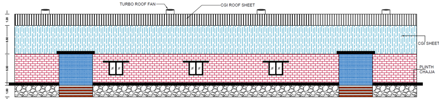
FRONT ELEVATION
